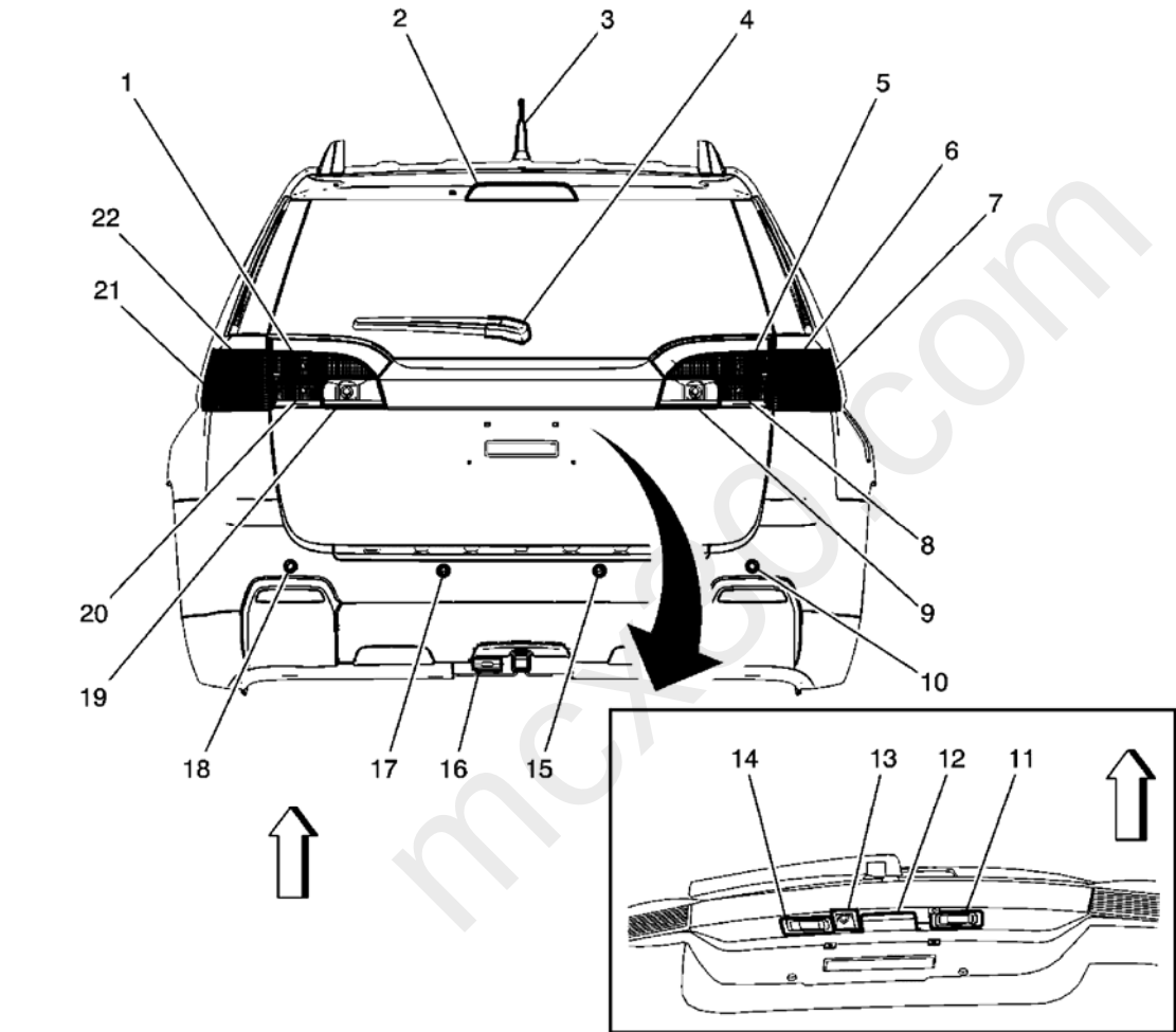
Fig. 5: Identifying Rear of Vehicle Components (GMC) Courtesy of GENERAL MOTORS CORP.
